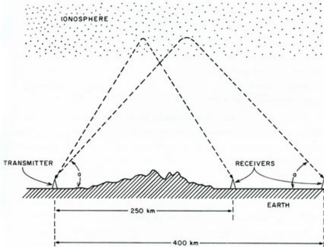
FIG. 6 HIGH-ANGLE RADIATION
