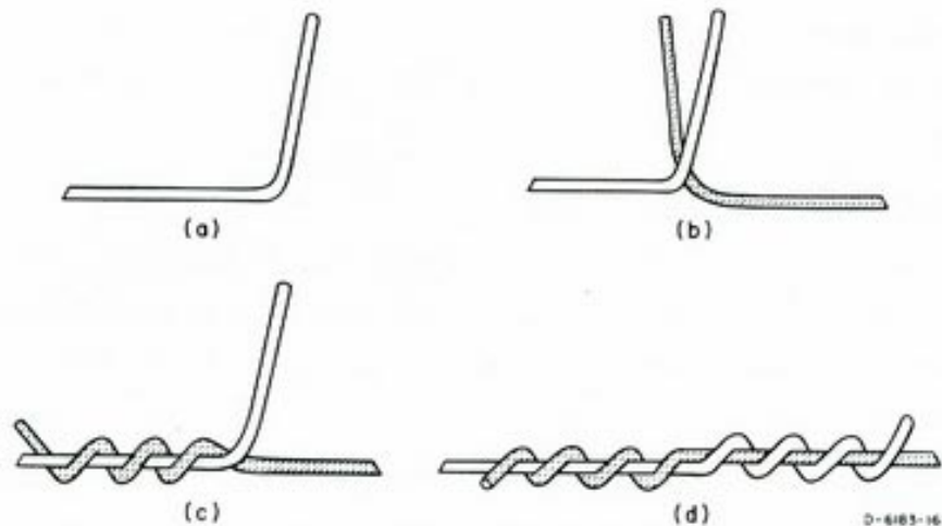
FIG. A-4 CORRECT WIRE SPLICE
