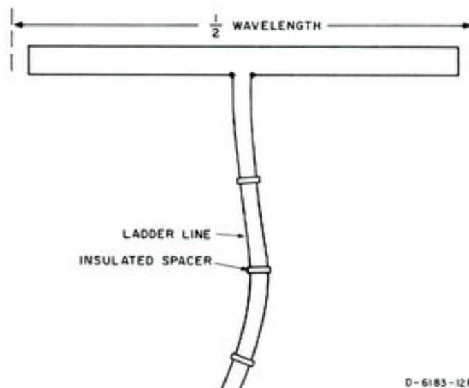
FIG. 12 FOLDED DIPOLE
