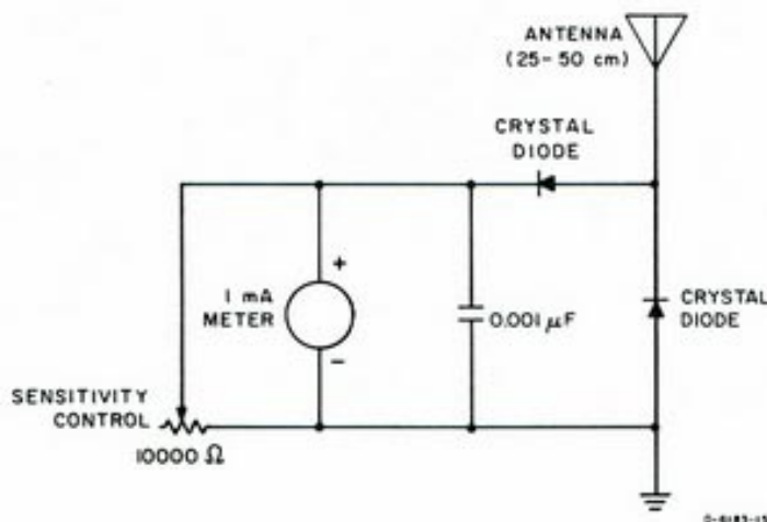
FIG. A-3 FIELD STRENGTH INDICATOR
