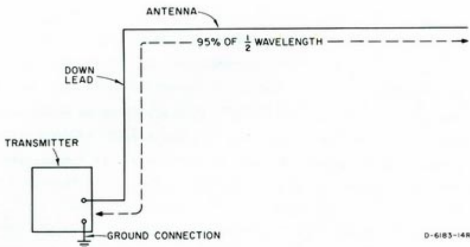
FIG. 15 SINGLE-WIRE ANTENNA
