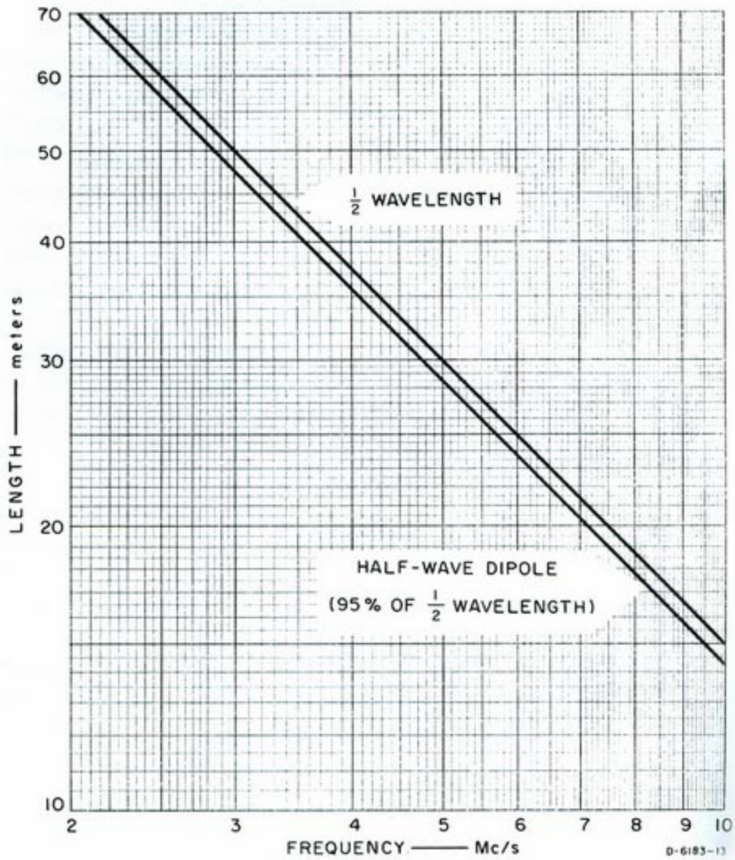
FIG. 13 LENGTH OF HALF-WAVE DIPOLE ANTENNA
