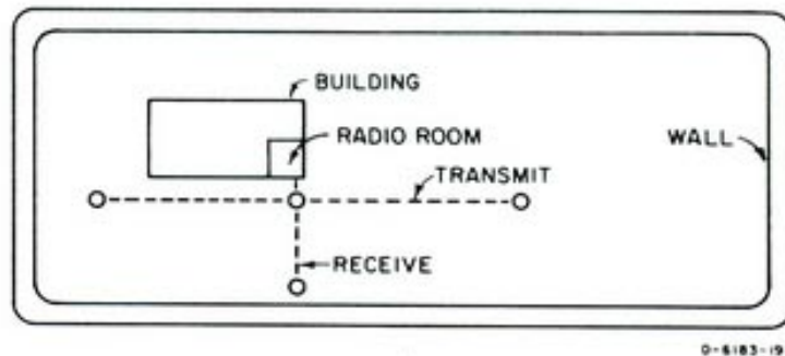
FIG. A-1 EXAMPLE OF ANTENNA POLE SITING
